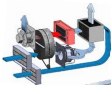
DFRIGO series operating principle
